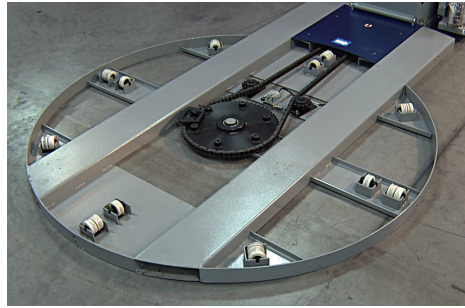
Structural steel plate and tube is used to provide a robust and durable base. Soft-start rotation prevents unstable loads from toppling when cycle begins.
